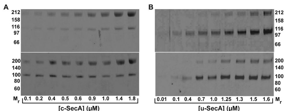
Figure 4. Signal peptide binding to SecA. Glutaraldehyde cross-linking was employed to assess signal peptide binding to c-SecA (A) and u-SecA (B) using a biotinylated model signal peptide. The presence of signal peptide was detected with streptavidin–horseradish peroxidase (bottom panels in A and B); signal peptide binds in a concentration-dependent manner primarily to dimeric c-SecA and monomeric u-SecA. The top gel panel in both (A) and (B) shows Coomassie Blue staining of the duplicate gel run in parallel.
