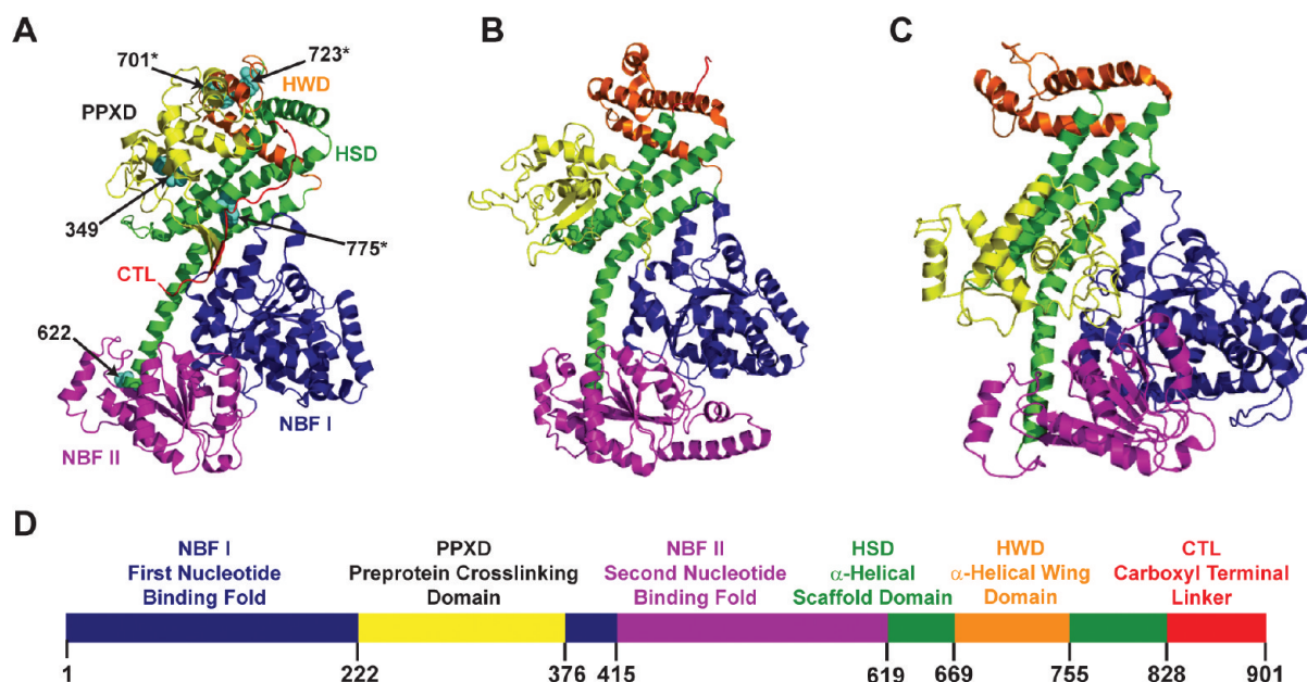
Figure 1. Domain organization and structural plasticity of the SecA PPXD. The overall domain organization of SecA in the three different crystal structures is similar, but the orientation of PPXD is different. (A) In the B. subtilis SecA structure 7 (PDB: 1M6N), the PPXD makes several intramolecular interactions with the HWD. The extreme C-terminal 40 residues are unresolved in this structure. The tryptophan residues corresponding to E. coli SecA Trps are shown in cyan spheres except for W519 and W541, which are located in a helical region of NBF II that is not present in B. subtilis SecA. Asterisks indicate the three tryptophan residues that contribute most to the overall SecA fluorescence. 22 (B) In the structure of monomeric B. subtilis SecA 15 (PDB: 1TF5) the PPXD no longer interacts with the HWD. The last 61 residues are unresolved in this structure. (C) In the structure of the SecA-SecYEG complex (PDB: 3DIN, only SecA structure is shown) from T. maritima 16 the PPXD has rotated more extensively, making contact with NBF II. The last 55 residues are unresolved in this structure. (D) Linear representation of the E. coli SecA sequence illustrating the six different domains, with the color scheme that we use throughout this paper.
