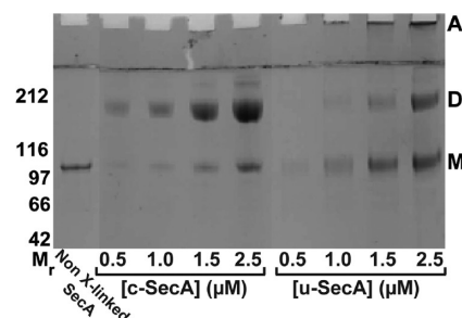
Figure 3. The oligomeric state of the c-SecA and u-SecA monitored by glutaraldehyde cross-linking followed by SDS-PAGE analysis. The different oligomeric forms of SecA (M, monomer; D, dimer; A, aggregates) are indicated on the right side of the gel. The concentrations of c-SecA and u-SecA are shown below the gel. The diffuse nature of the cross-linked band arises from intramolecular cross-linking occurring along with the intersubunit cross-linking. The molecular weight standards, M_r , are shown in kDa in this and all other figures.
