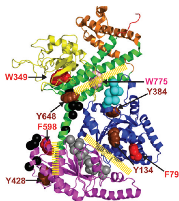
Figure 7. Structural interpretation of conformationally diagnostic accessibility data for u-SecA from limited proteolysis, fluorescence, and literature results. Residue positions that were cut by \alpha -CT in c-SecA and u-SecA based on the data shown in Figure 6B are mapped onto the NMR structure of E. coli SecA (PDB: 2VDA). Spacefill residues colored as brown and red represent class II and III cleavage sites, respectively, and W775 is shown in light pink spacefill. Class I sites are shown in spacefill in the same color as the domain to which they belong. SecA residues that are reported to undergo conformational change in the presence of its natural ligands are shown with their C\alpha atoms in spacefill: Motif IV (in cyan), buried in c-SecA, is reported to become accessible to make contact with SecYEG 56 in translocation-active SecA. Motif VI (in gray) is a highly mobile region in c-SecA by NMR studies. 9,47 Residues in black represent residues that become more mobile based on EPR labeling when SecA interacts with phospholipids. 48 Interdomain interfaces that we propose to be disrupted in the transition from c-SecA to u-SecA are indicated by yellow hatched lines.
