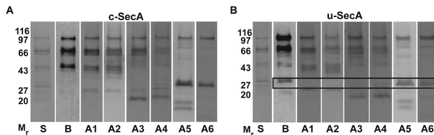
Figure 8. Signal peptide photo-cross-linking to c-SecA (A) and u-SecA (B). Equimolar amounts of c-SecA or u-SecA and signal peptide were cross-linked using a photoactivatable cross-linker, as described in the text. S, B, and A1–A6 denote respectively Coomassie Blue visualization of the gel, enhanced chemiluminescence detection of SecA cross-linked to biotinylated signal peptide, and Western blotting with the six region-specific SecA antibodies. Note that signal peptide cross-linked significantly to a 30 kDa band in u-SecA that is also recognized by the two C-terminal SecA antibodies, A5 and A6.
